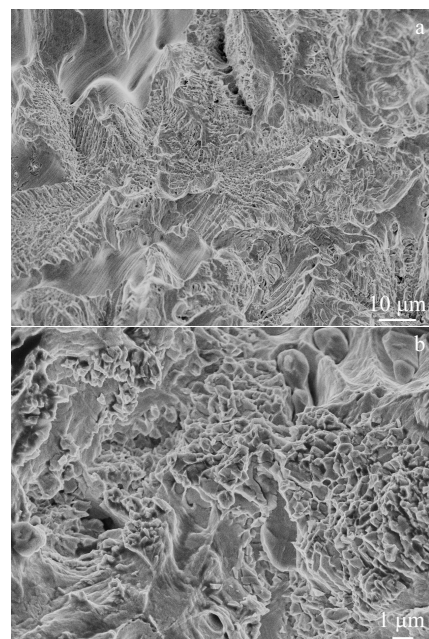
Fig.8 SEM morphologies of tensile fracture of 316L ASSs prepared with excess fraction \text{Fe}_2\text{O}_3 of 5.0%: (a) stream patterns and (b) dimpled fractures
