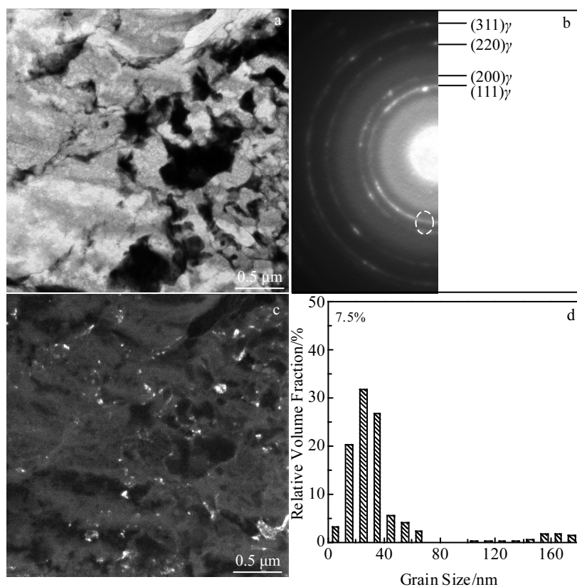
Fig.6 TEM analysis results of 316L ASSs prepared with excess fraction \text{Fe}_2\text{O}_3 of 7.5%: (a) bright-field image, (b) corresponding SAED pattern, (c) dark-field image and (d) histogram of grain size distribution determined from dark field images (dotted circle in SAED pattern indicates the operating spots of the dark-field image)
