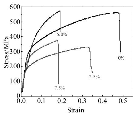
Fig.7 Tensile stress-strain curves of 316L ASSs prepared with different excess fractions of \text{Fe}_2\text{O}_3
