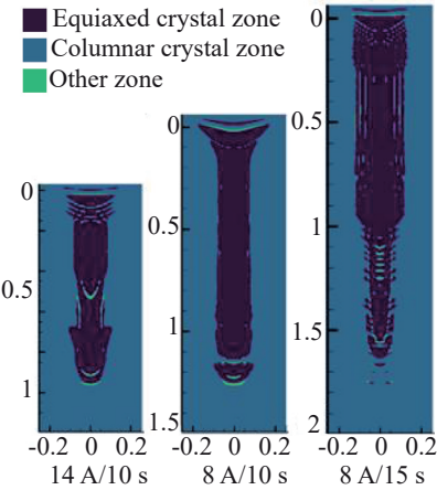
图11 预测的Ti-1023铸锭不同区域形貌分布 Fig.11 Distribution maps of different morphological zones of the predicted Ti-1023 ingots
