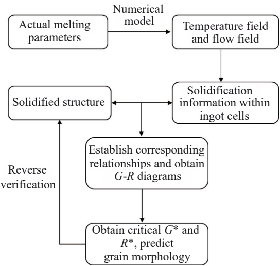
图9 晶粒形态预测流程图 Fig.9 Flowchart for grain morphology prediction
