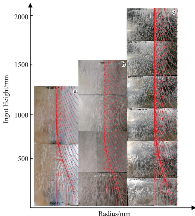
图7 不同磁场条件下制备的Ti-1023合金铸锭纵截面晶粒生长方向 Fig.7 Grain growth direction in longitudinal macrostructures of Ti-1023 alloy ingots under different magnetic field conditions: (a) 14 A/10 s, (b) 8 A/10 s, and (c) 8 A/15 s
