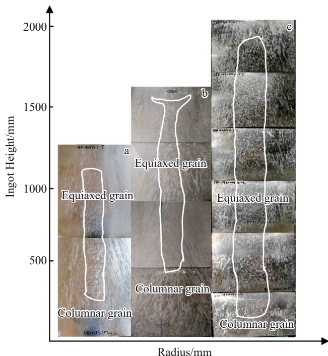
图6 不同磁场条件下制备的Ti-1023合金铸锭纵截面宏观组织 Fig.6 Longitudinal macrostructures of Ti-1023 alloy ingots under different magnetic field conditions: (a) 14 A/10 s, (b) 8 A/10 s, and (c) 8 A/15 s
