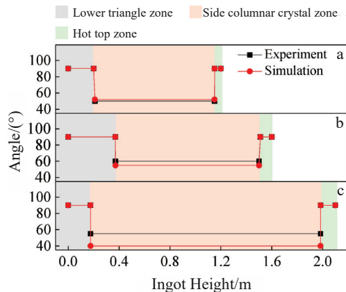
图8 不同磁场条件下实际与模拟预测的铸锭晶粒生长方向对比 Fig.8 Comparison of the actual and simulated predicted grain growth directions of ingots under different magnetic field conditions: (a) 14 A/10 s, (b) 8 A/10 s, and (c) 8 A/15 s
