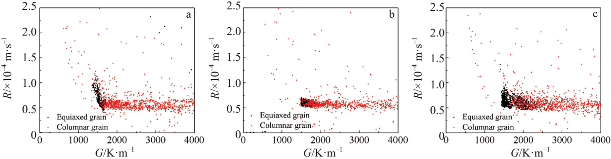
图10 晶粒形态分布图谱( R-G ) Fig.10 Maps of the distribution of different morphological zones ( R-G ): (a) 14 A/10 s, (b) 8 A/10 s, and (c) 8 A/15 s
